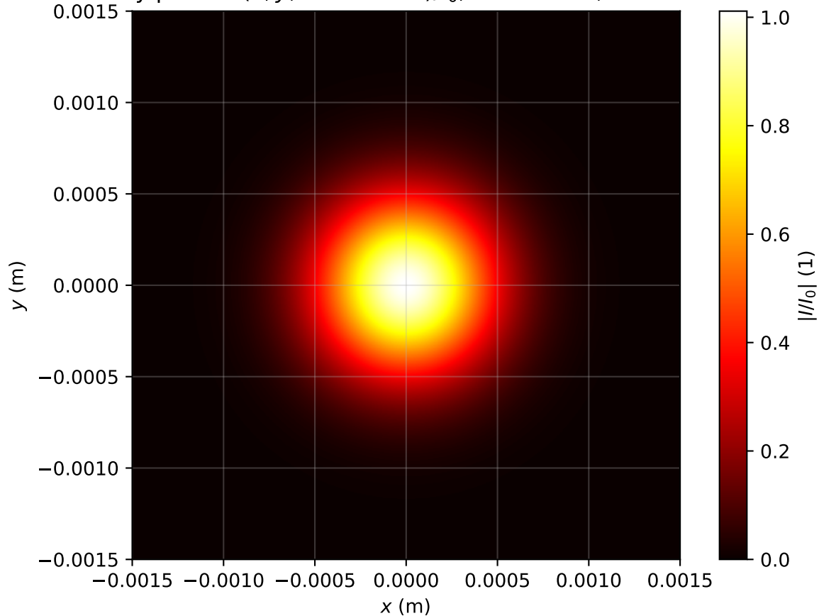
Intensity profile I(x, y, z = 0.159m)/I_0 , Pin=0.7Pcr, artificial time
